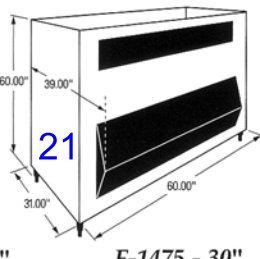
F-1475 - 30" or 48" ice maker
